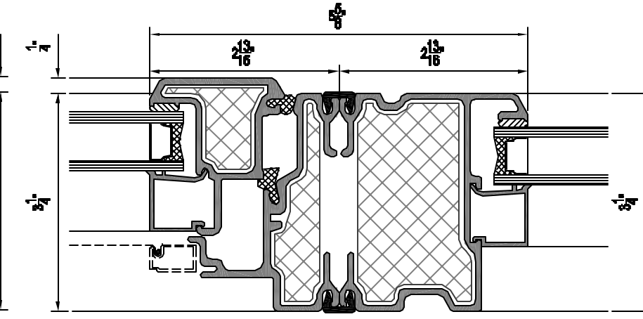
6 INTERMEDIATE DETAIL 325
