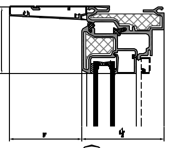
F #115 3-1/4 325
