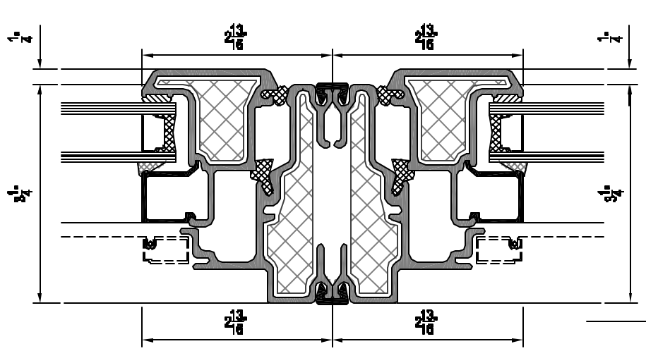
4 INTERMEDIATE DETAIL 325
