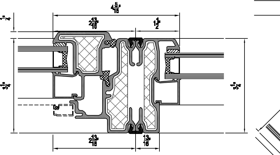
5 INTERMEDIATE DETAIL 325
