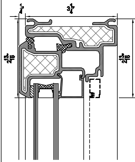
1 HEAD DETAIL 325
