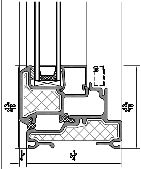
2 SILL DETAIL 325
